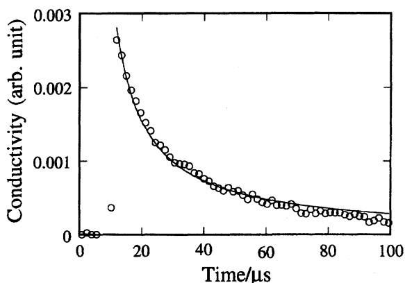
Fig. 3. A decay profile of the transient electric conduction measured on excitation of DCA ( 1 \times 10^{-4} \text{ M} ) with 425-nm laser pulses in the presence of HMB (0.1 M) in acetonitrile. The solid line is fitted with a decay rate constant of 3.6 \times 10^7 \text{ M}^{-1} \text{ s}^{-1} .
